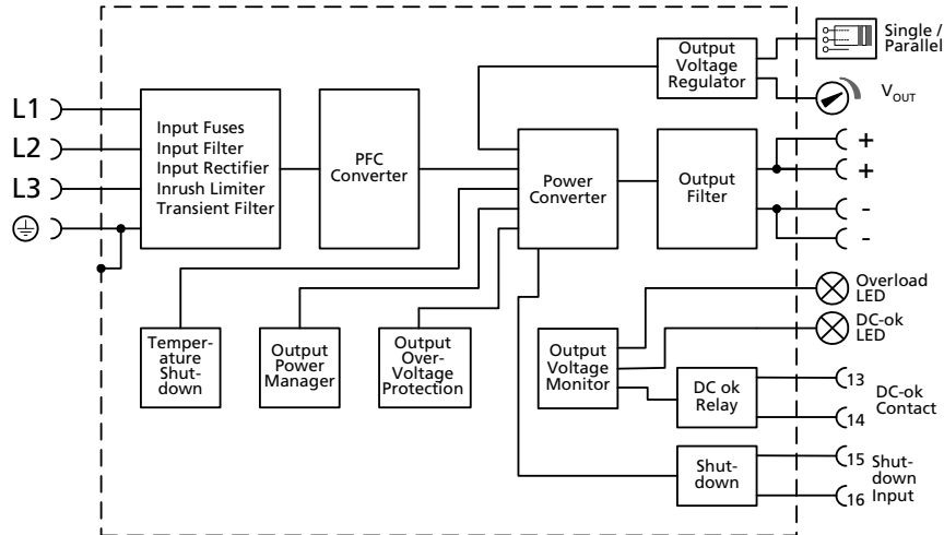
Fig. 13-1 Functional diagram
