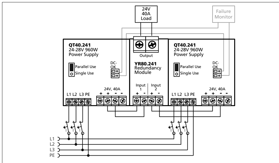
Fig. 23-1 Typical 1+1 Redundant configuration for 40A with a dual redundancy module
