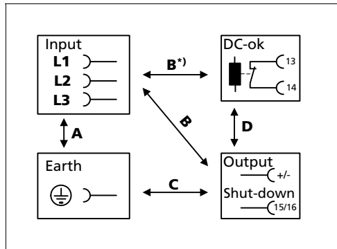
Fig. 20-1 Dielectric strength
