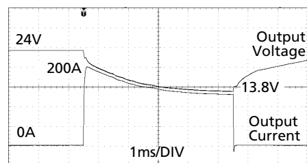
Fig. 25-4 Peak load with 5x the nominal current for 5ms, typ.
