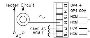
Heater Current Monitor
